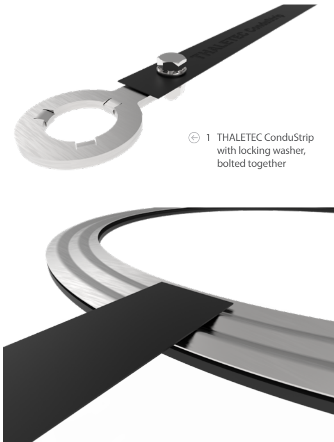
③ Flange gasket with inserted ConduStrip
